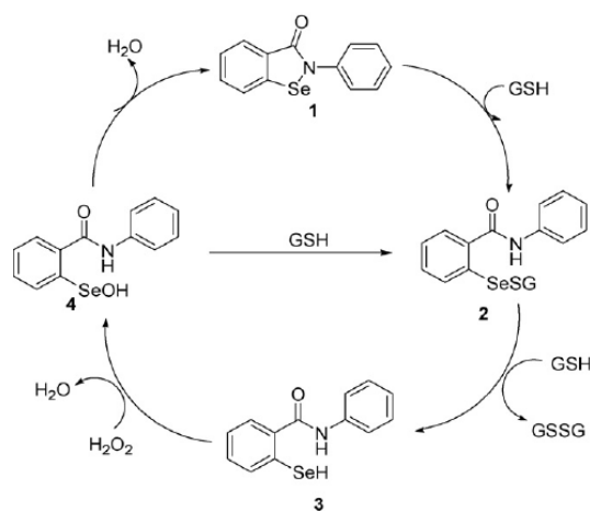
Fig. 5. Catalytic anti-oxidant cycle of ebselen.
